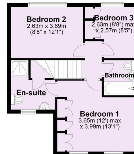
First Floor Approx. 42.1 sq. metres (453.3 sq. feet)
